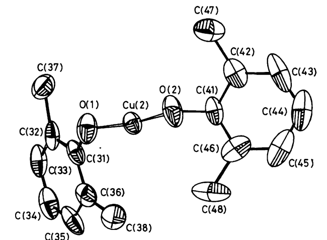
Figure 2. An ORTEP view of the anion [(2,6\text{-Me}_2\text{C}_6\text{H}_3\text{O})_2\text{Cu}]^- in complex (5). Bond distances (Å): Cu(2)–O(1) 1.806(6), Cu(2)–O(2) 1.798(8), C(31)–O(1) 1.319(11), C(41)–O(2) 1.323(10); bond angles (°): O(1)–Cu(2)–O(2) 169.8(3), Cu(2)–O(1)–C(31) 137.0(5), Cu(2)–O(2)–C(41) 135.2(5).
